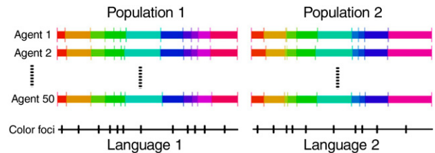
Fig. 1. An example of the results from the simulations of two different populations with the human JND ( d_{\min}(x) ) function. After 10^4 games, the pattern of categories and associated color terms are stable throughout the population. Different individuals in one population have slightly different category boundaries, but the agreement is almost perfect (larger than 90%). As for each category, a focal color point is defined as the average of the midpoints of the same category across individuals in the population. Different populations may develop different final patterns.
